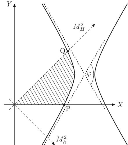
Fig. 1. The region of admissible values of M_h^2 if h is assumed to be the lightest scalar
