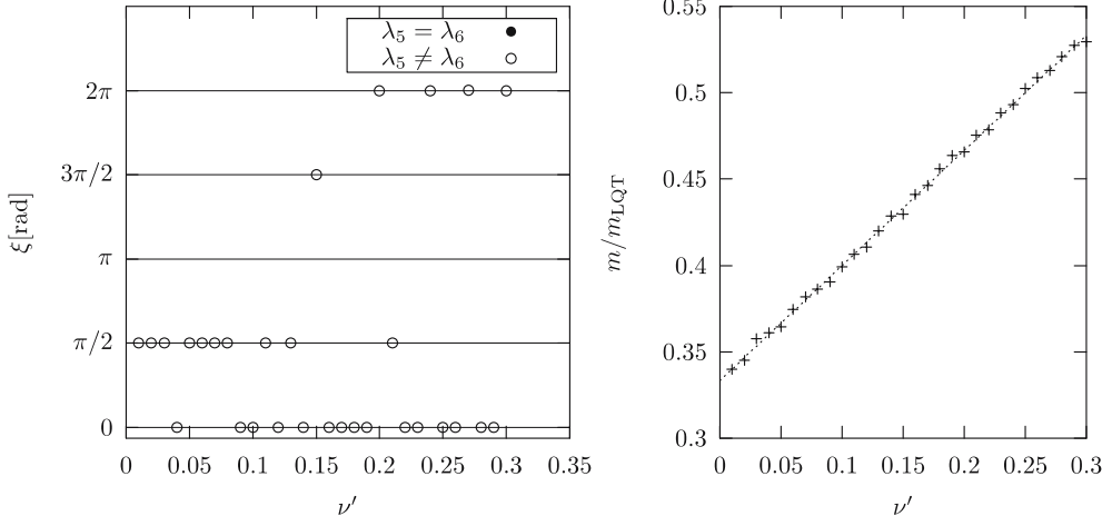
Fig. 4. Lightest scalar mass, with theoretical estimate (51)
