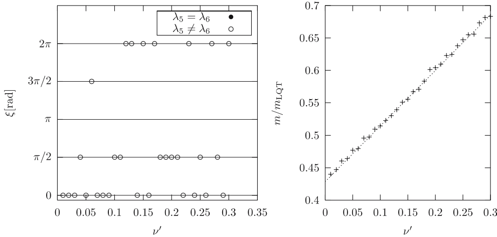
Fig. 6. Lightest neutral boson with theoretical estimate (53)
