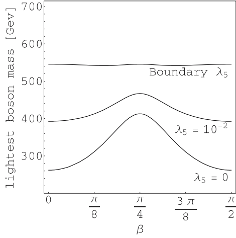
Fig. 2. Dependence of lightest boson mass on \beta
