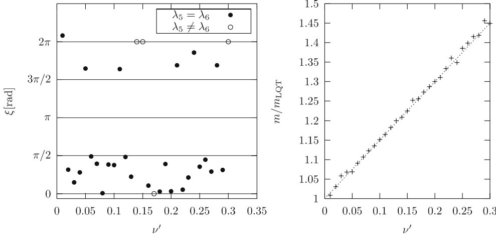
Fig. 3. Charged Higgs boson, with theoretical estimate (36)
