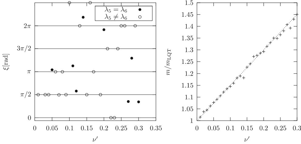
Fig. 5. Heaviest neutral Higgs boson, with theoretical estimate (44) or (38)
